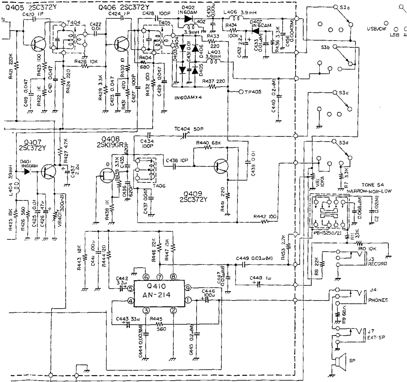
FRG-7 CIRCUIT DIAGRAM
