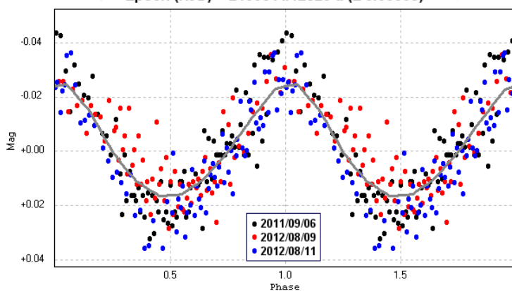
2MASS J21431348+0109335 P = 0.17699 d ( \pm 0.00024) Epoch (HJD) = 2455811.42825 d ( \pm 0.00605)
