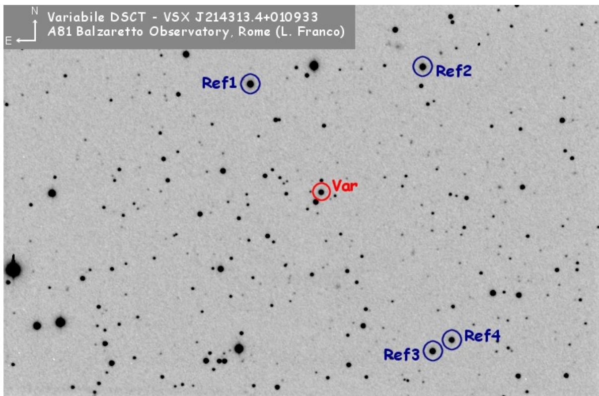
2MASS J21431348+0109335 P = 0.17699 d ( \pm 0.00024) Epoch (HJD) = 2455811.42825 d ( \pm 0.00605)
