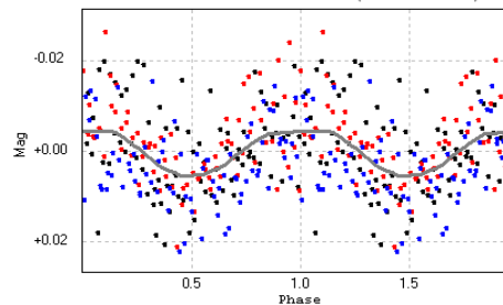
2MASS J21431348+0109335 (P = 0.13784 d)
